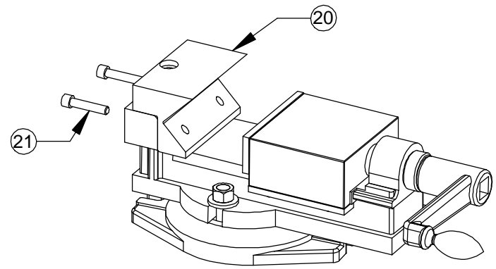
1100-U Upgraded Vise
